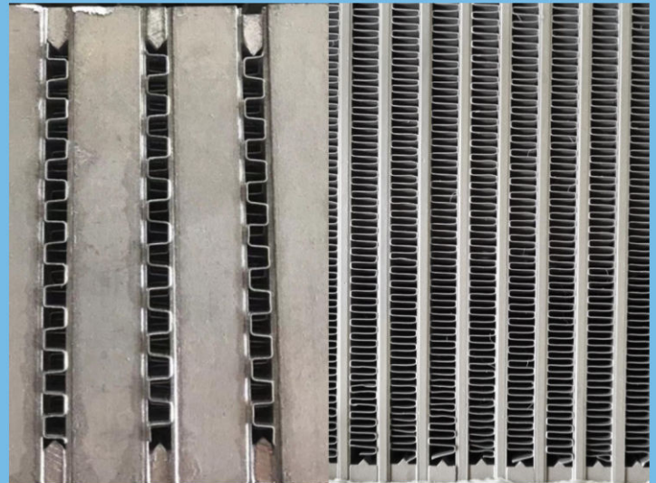
Plate & Bar Aluminum Oil Cooler Core
