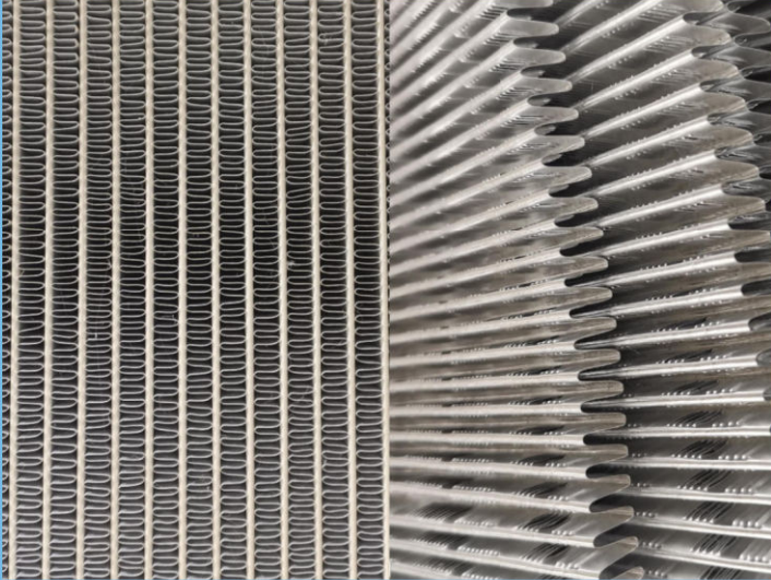
Tube & Weave Fin Aluminum Radiator Core
