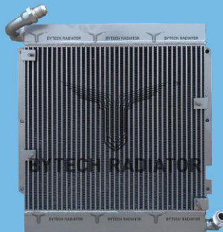
PC60-5 Oil Cooler
