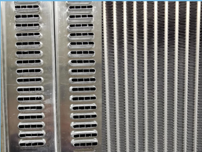
Tube & Weave Fin Aluminum Intercooler Core
